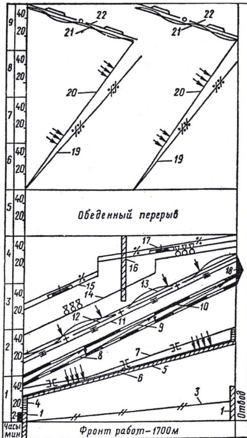
Fig 4.1.2 – 1 Main work schedule in the major repair works on track
