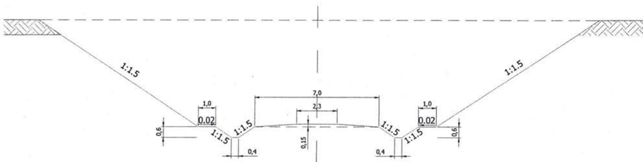
Fig. 2.1 – 2 Standard cutting cross section
