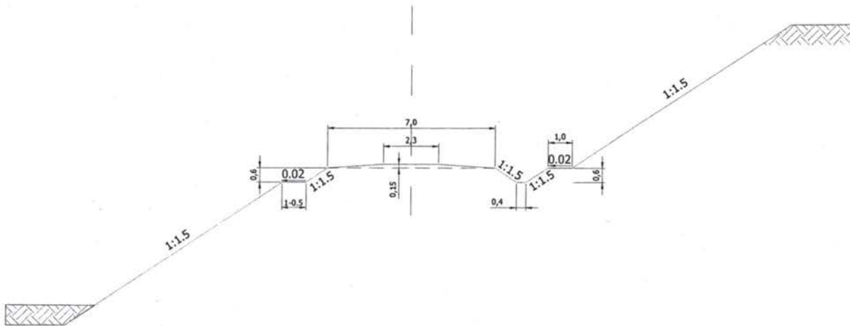
Fig. 2.1 – 3 Standard semi-cut cross section
