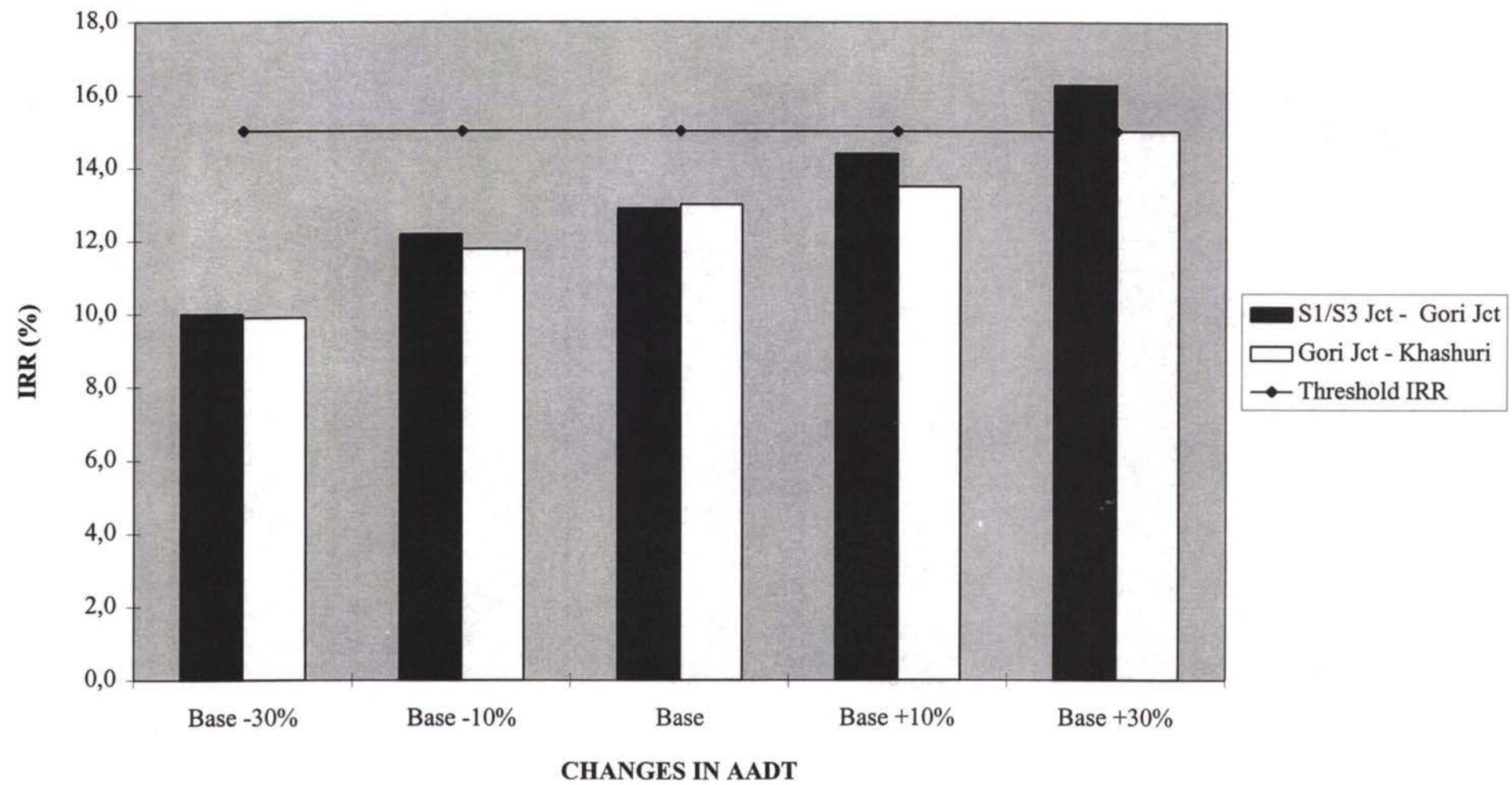
FIGURE 8.2 SENSITIVITY OF IRR TO CHANGES IN BASE YEAR TRAFFIC
